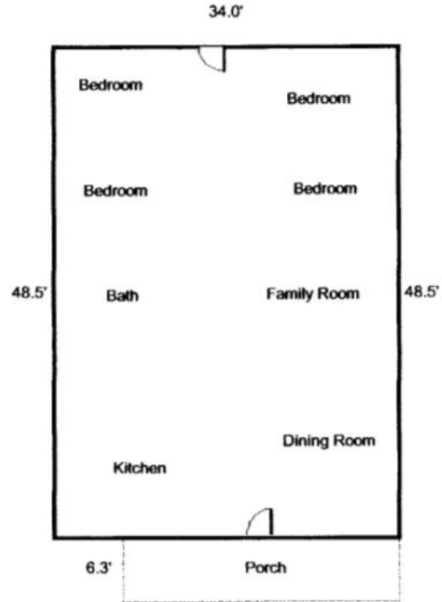
Front Second Floor
